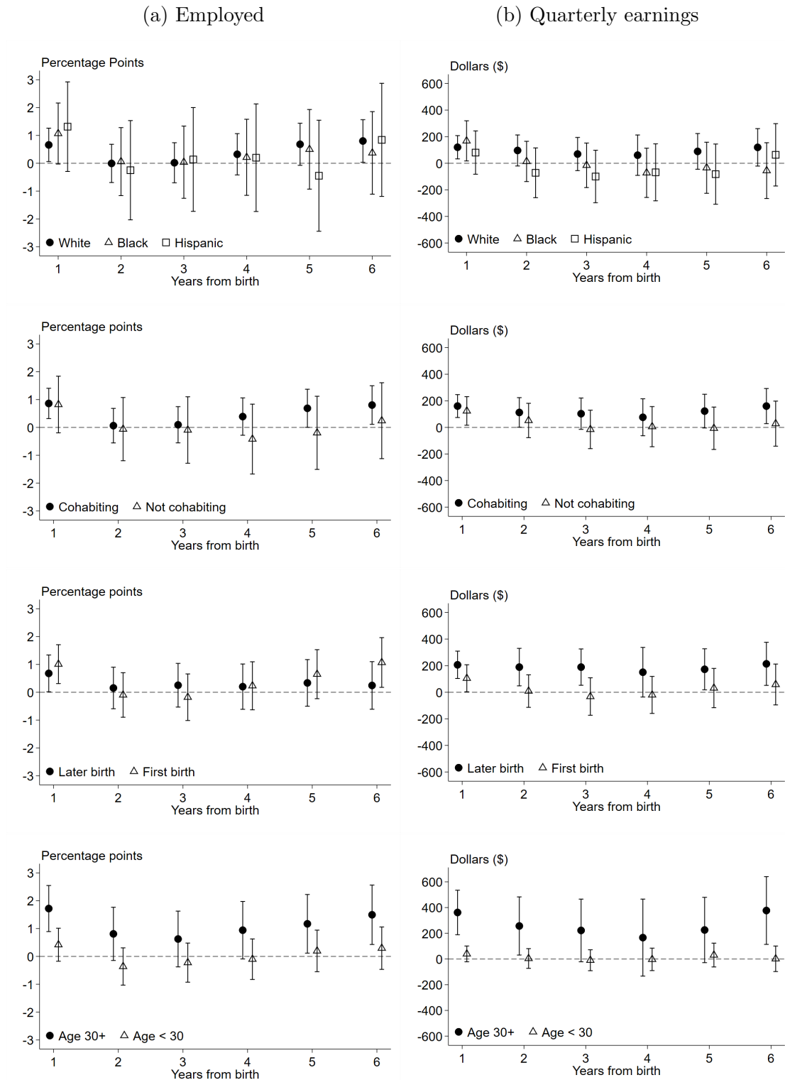
Figure 7: Heterogeneity analysis
